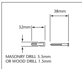
SCREWS (AND PLASTIC ANCHORS FOR MASONRY) 2 PER BOX
