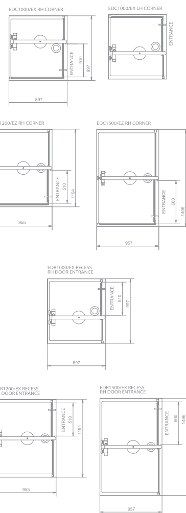
Above drawings show right hand illustrations only for models 1200 and 1500. For left hand, reverse illustrations.
