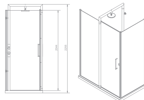
Above illustration shows a left hand corner. On corner installations, door always closes against side panel side.
